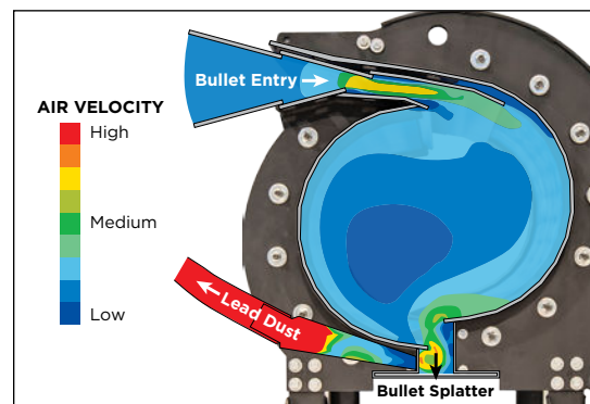
Side View of Vortex Chamber Airflow Analysis
